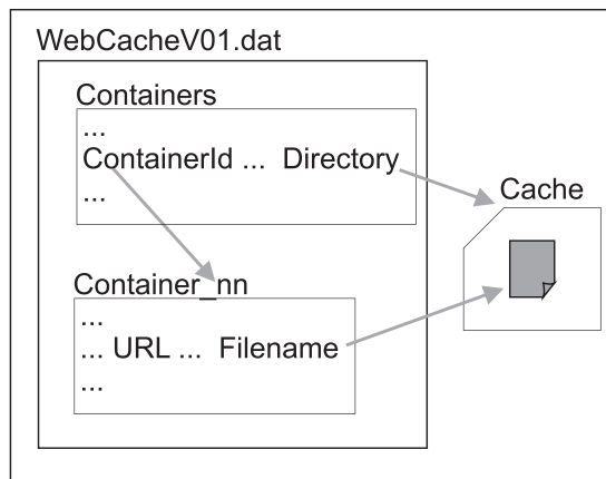
Fig. 2. Overview of Cache Data Structures. The Containers table acts as an index into a series of Container_nn tables and specifies the directory path to the related cache directory; individual records in the Container_nn table specify the cached filename.
