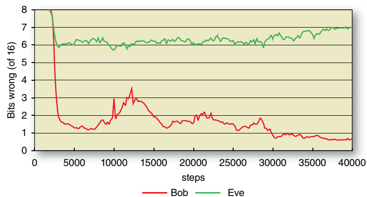
FIGURE 5.6 Effectiveness of Bob and Eve in receiving and decrypting messages over time.
