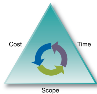
FIGURE 13.6 Triple constraint.
