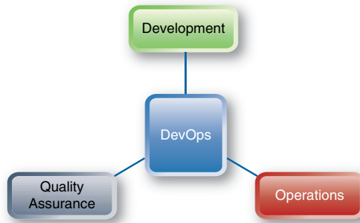
FIGURE 13.5 DevOps
