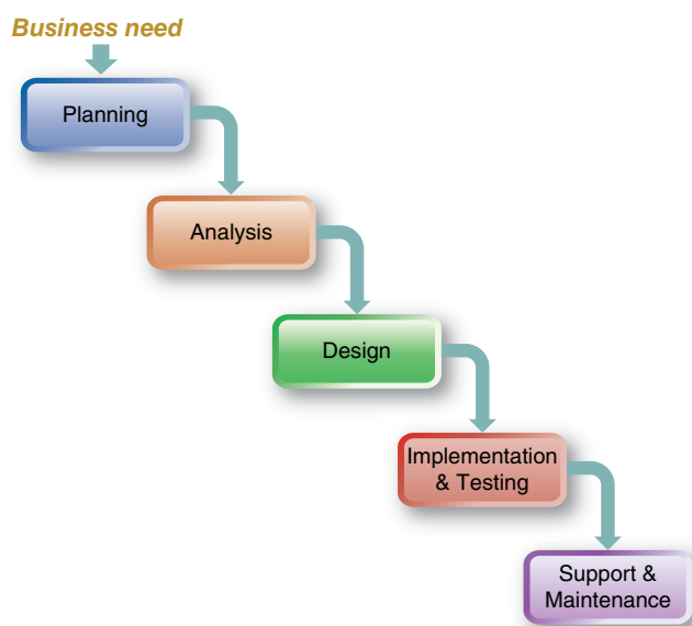
FIGURE 13.2 Waterfall Method.
