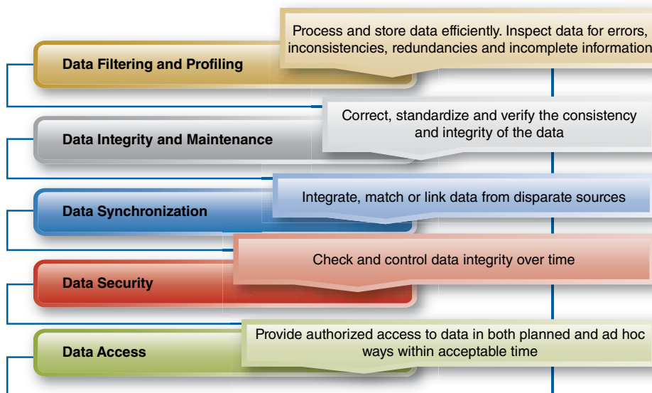
FIGURE 3.5 DBMS functions.
